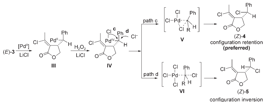
Scheme 3. Possible \text{Pd}^{\text{II}}/\text{Pd}^{\text{IV}} mechanisms for the formation of a C–Cl bond.
